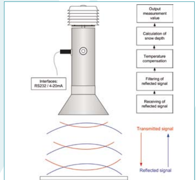
Fig. 1: Signal processing by the USH-8 snow depth sensor.
